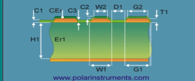
Coated Coplanar Strips With Ground 1B
