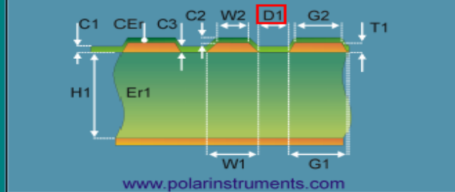
Coated Coplanar Strips With Ground 1B
