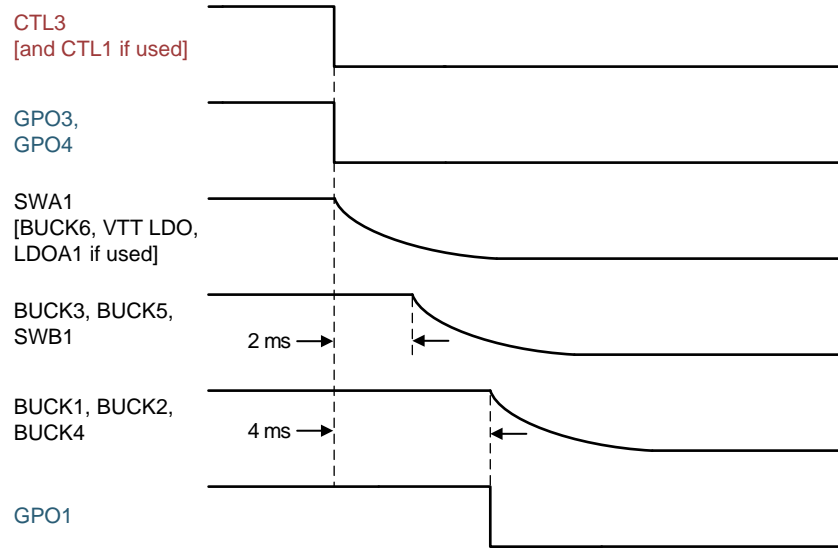
Figure 6-5. TPS6508640 Power-Down Sequence
