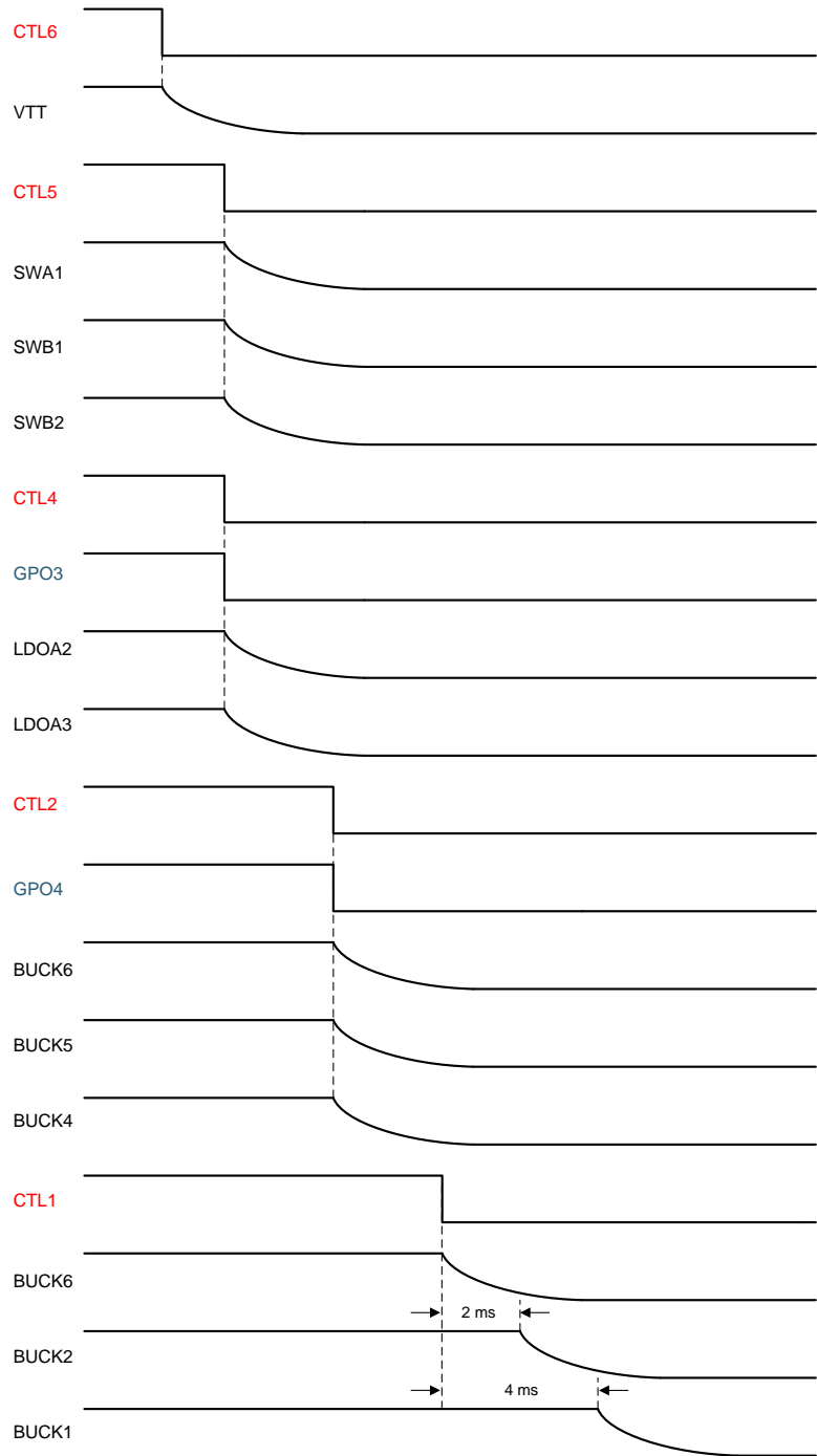
Figure 6-25. Generic Power-Down Sequence Example
