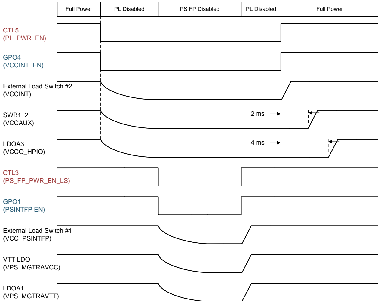
Figure 6-13. TPS6508641 Low Power States
