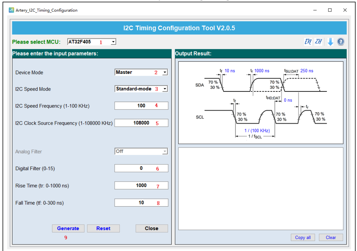
图 13. Artery I2C Timing Configuration
